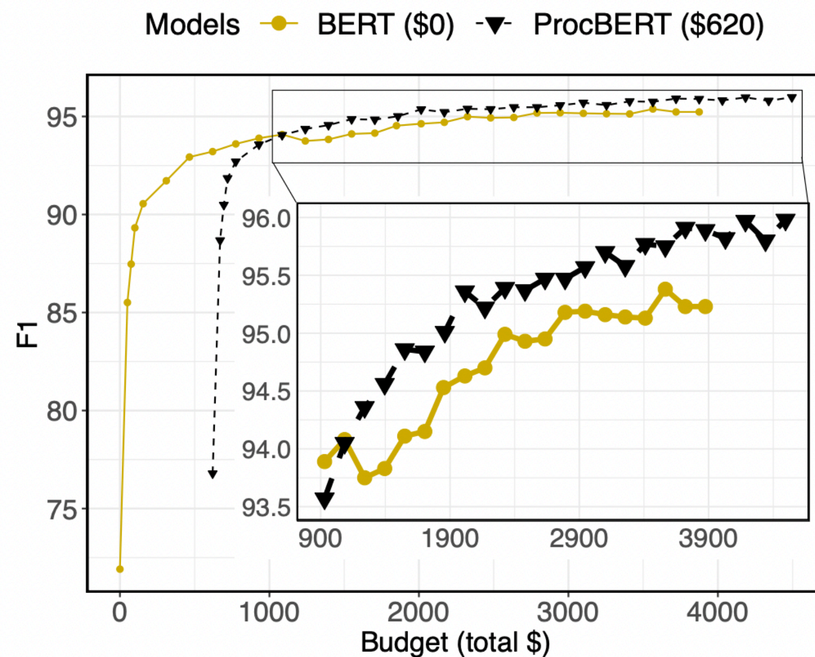
(a) PUBMEDM&M \Rightarrow CHEMSYN
